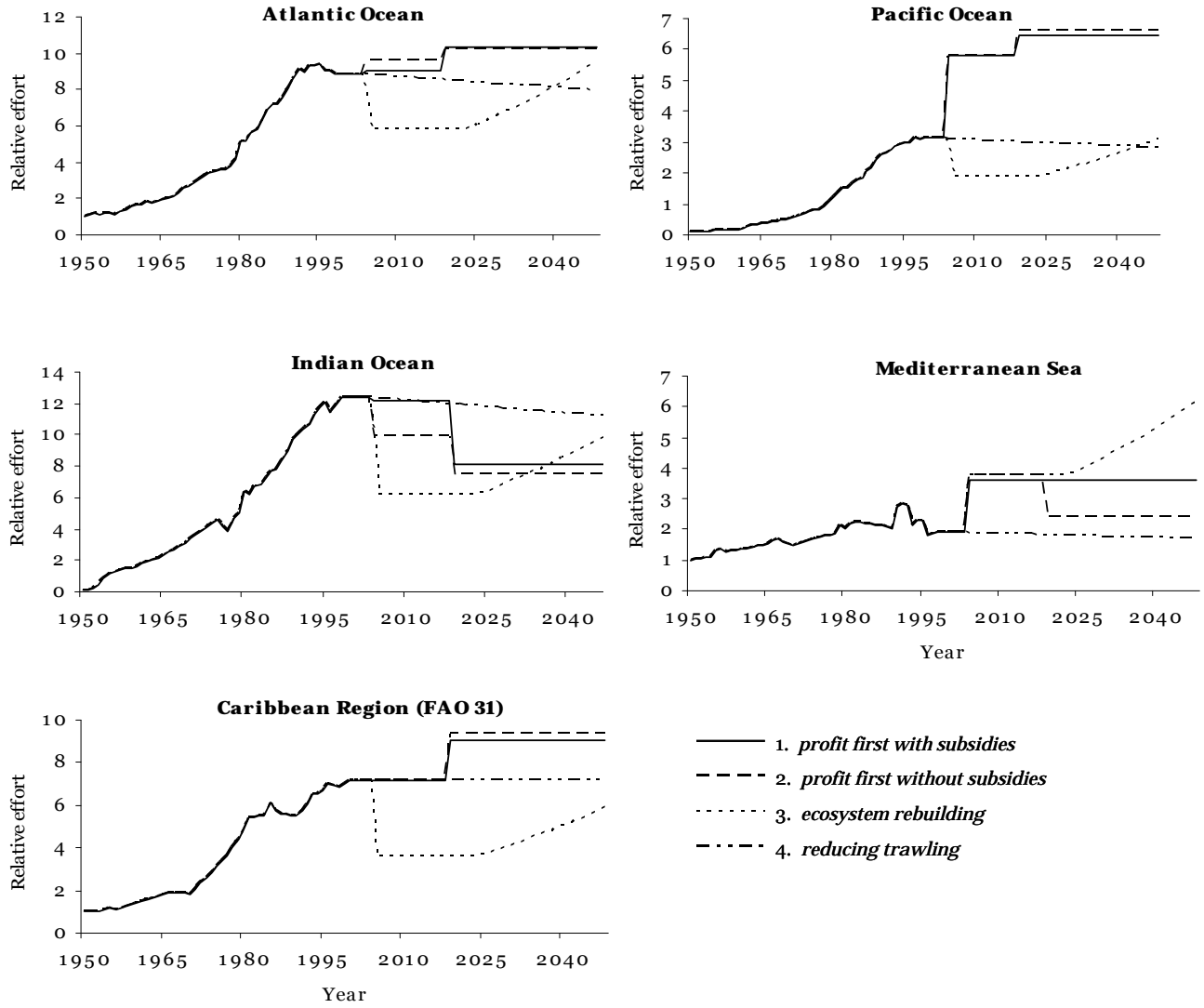
Figure 11. Average demersal effort by ocean for the four IAASSTD policy scenarios.
